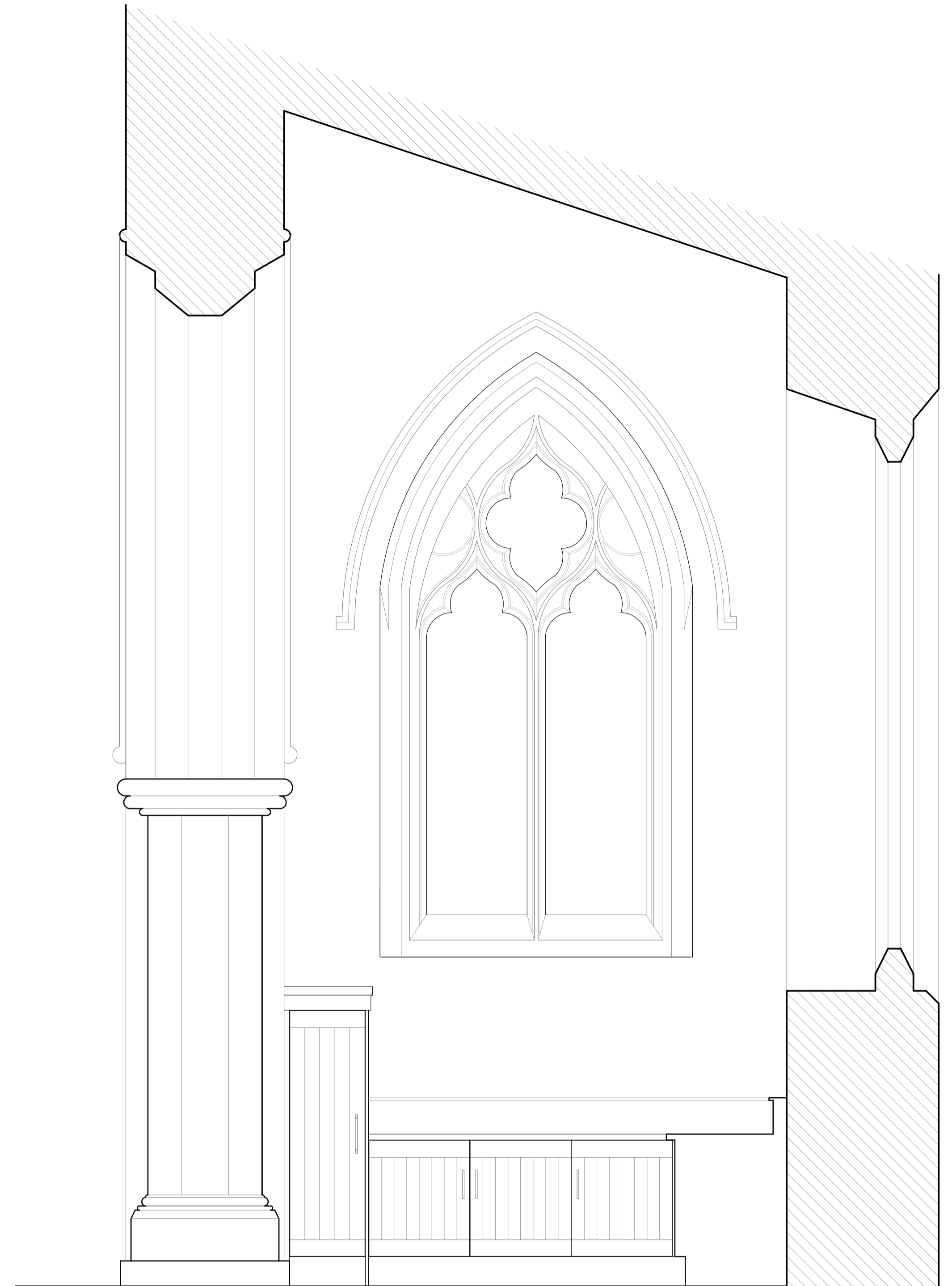
1:20 ELEVATION B-B AS PROPOSEED
