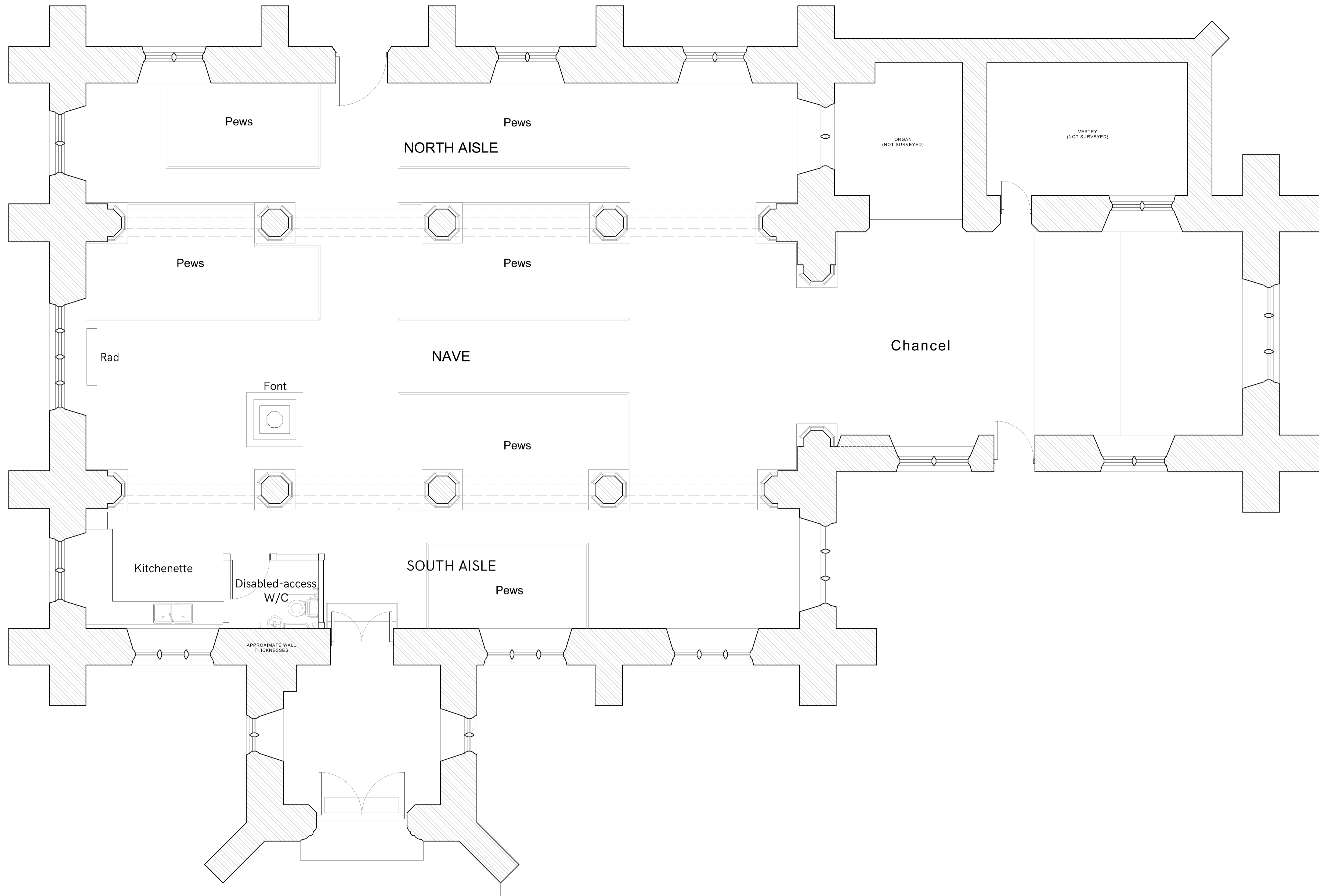
1:50 GROUND FLOOR PLAN AS EXISTING
