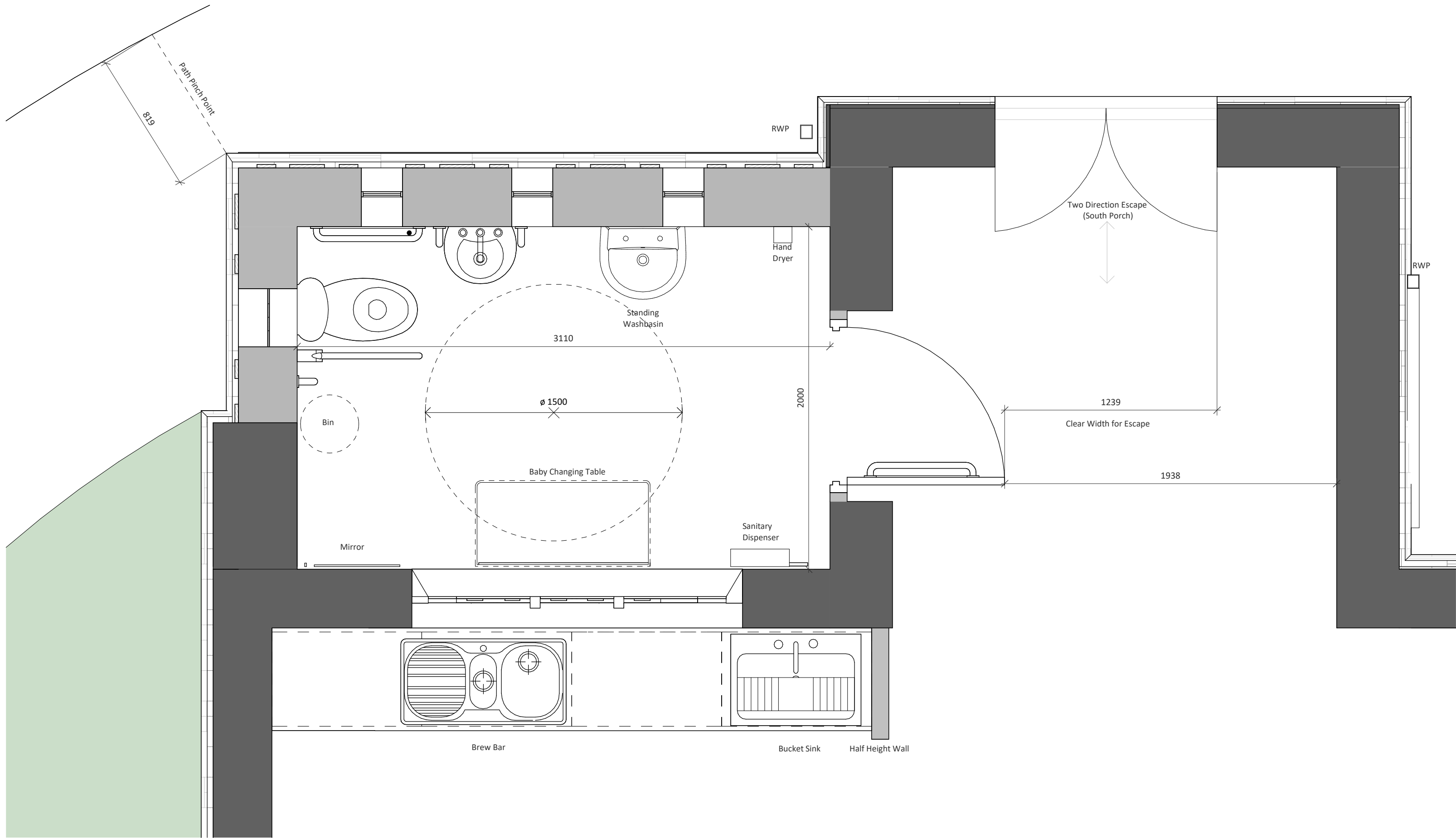
1 | PROPOSED WC PLAN SCALE: 1 : 20
