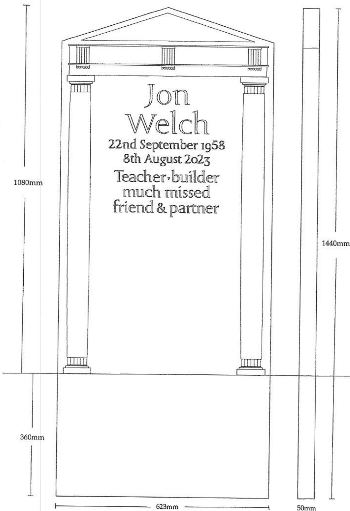
Headstone to Jon Welch on Cumbrian Green Slate, Front & Side Elevations Scale 1:5.5
